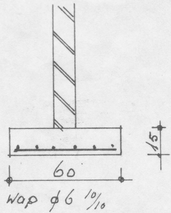
FUNDERING DETAIL
